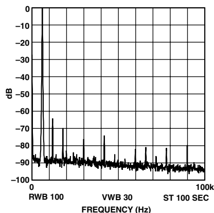
TPC 12. f_{MCLK} = 25 MHz, f_{OUT} = 6 kHz, Frequency Word = 000FBA9
