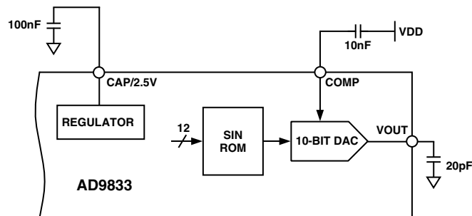
Figure 1. Test Circuit Used to Test Specifications
