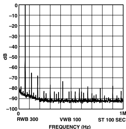
TPC 13. f_{MCLK} = 25 MHz, f_{OUT} = 60 kHz, Frequency Word = 009D495
