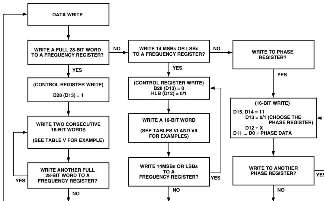
Figure 9. Data Writes
