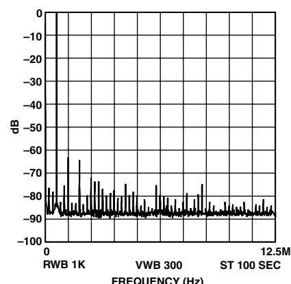
TPC 14. f_{MCLK} = 25 MHz, f_{OUT} = 600 kHz, Frequency Word = 0624DD3
