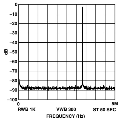
TPC 11. f_{MCLK} = 10 MHz, f_{OUT} = 3.33 MHz = f_{MCLK}/3 , Frequency Word = 5555555
