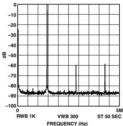
TPC 10. f_{MCLK} = 10 MHz, f_{OUT} = 1.43 MHz = f_{MCLK}/7 , Frequency Word = 2492492
