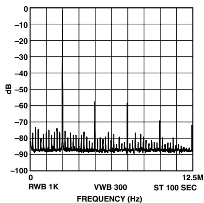
TPC 15. f_{MCLK} = 25 MHz, f_{OUT} = 2.4 MHz, Frequency Word = 189374D
