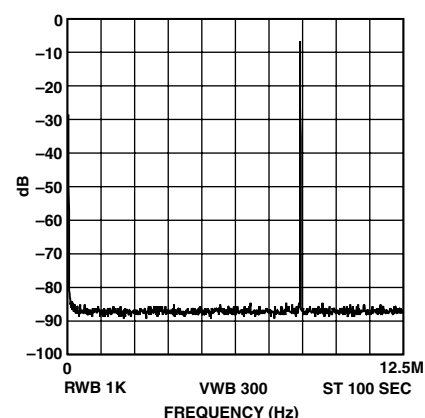
TPC 17. f_{MCLK} = 25 MHz, f_{OUT} = 8.333 MHz = f_{MCLK}/3 , Frequency Word = 5555555
