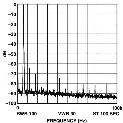
TPC 9. f_{MCLK} = 10 MHz, f_{OUT} = 2.4 kHz, Frequency Word = 000FBA9
