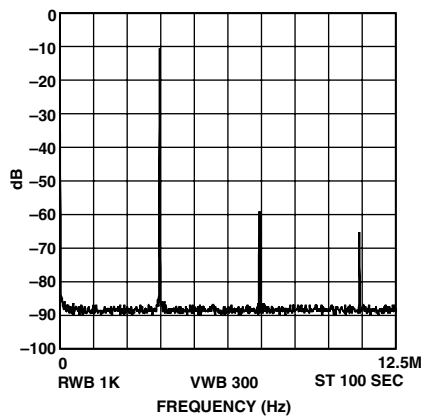
TPC 16. f_{MCLK} = 25 MHz, f_{OUT} = 3.857 MHz = f_{MCLK}/7 , Frequency Word = 2492492
